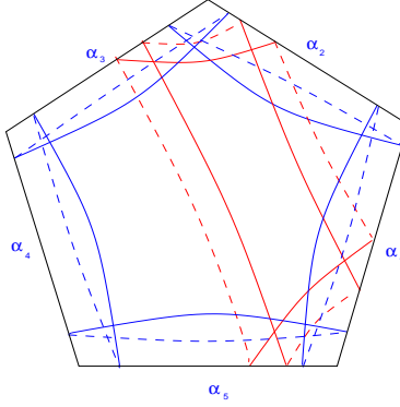
FIGURE 1. The set Y = A = \{\alpha_1, \dots, \alpha_5\} is the rigid set \mathfrak{X}(S_{0,5}) identified in [12, 1], and is a closed string of twistable Farey neighbors. The red curves in the picture are f_{\alpha_1}(\alpha_2), f_{\alpha_2}(\alpha_1) , for the twistable pair \alpha_1, \alpha_2 . The automorphism group of Y_A that fixes Y pointwise is generated by an orientation-reversing involution \sigma : S_{0,5} \rightarrow S_{0,5} that fixes \alpha_i and interchanges f_{\alpha_i} and f_{\alpha_{i+1}} , for all i \pmod{5} .
