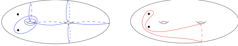
FIGURE 10. Determining the curve \gamma_1 .
