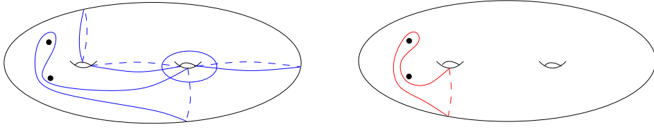
FIGURE 11. Determining the curve H_{e^{i,i+1}}(\alpha_0^i) .
